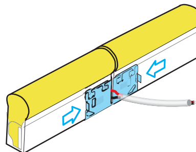
DIY snap splice connector (IP67 Only)
